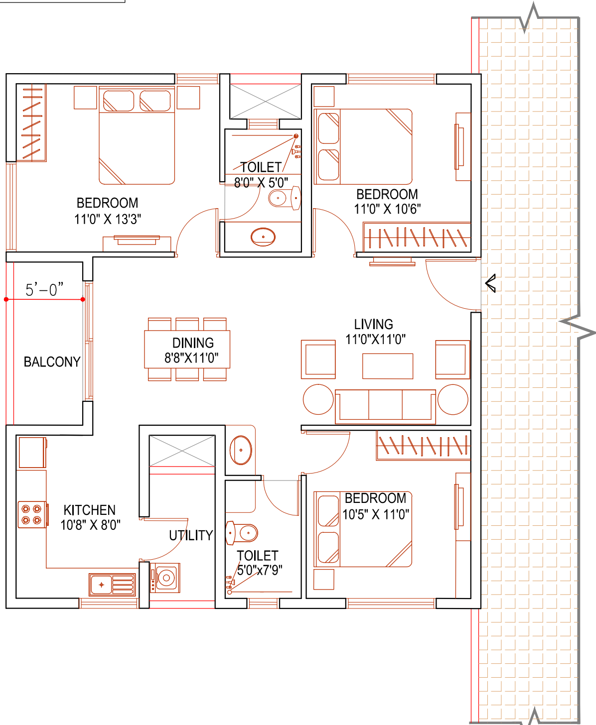
UNIT PLAN - TYPE 2B (3 - BHK NORTH FACING) Saleable Area - 1340 Sft
