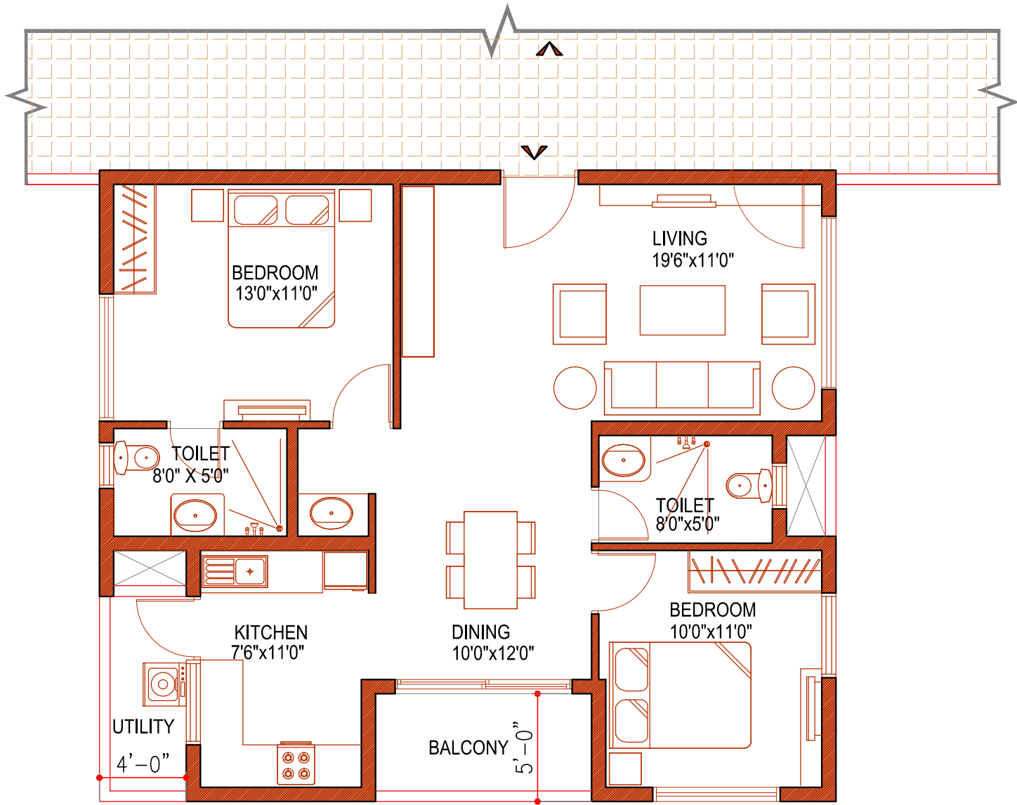
UNIT PLAN - TYPE 3A (2 - BHK WEST FACING) Saleable Area - 1245 Sft
