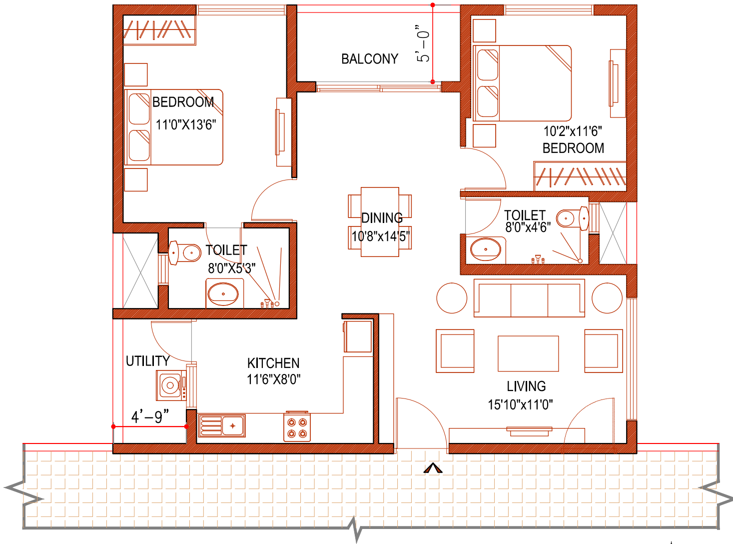
UNIT PLAN - TYPE 3 (2 - BHK EAST FACING) Saleable Area - 1235 Sft
